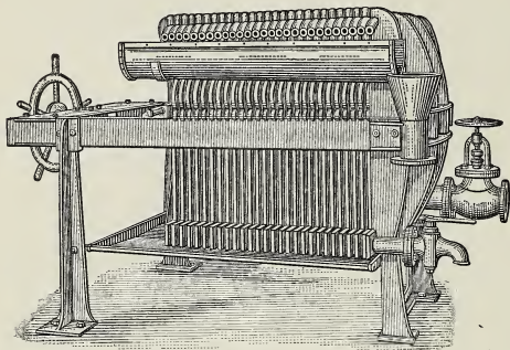
FIG. 29.—Filter-press.
